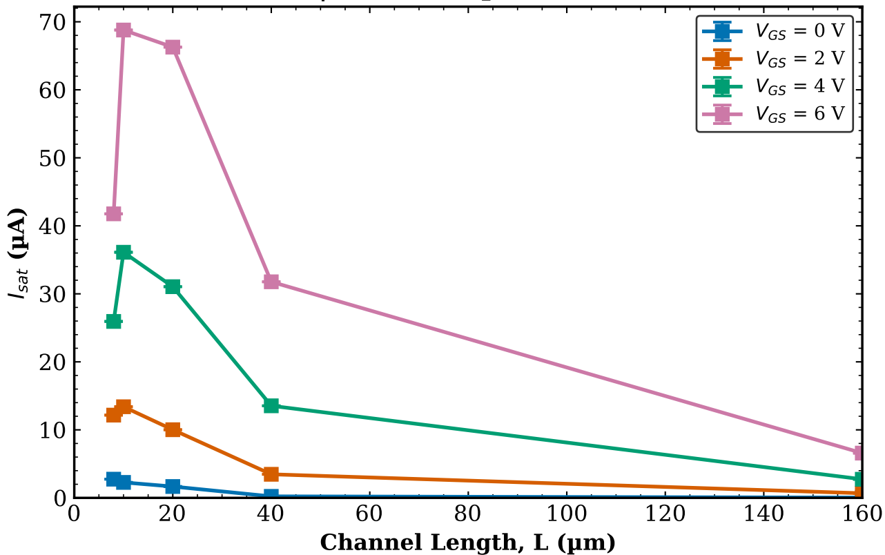
TFT1 Transistor 1 I_{sat} vs L | W = 100 \mu\text{m} (mean \pm std)
